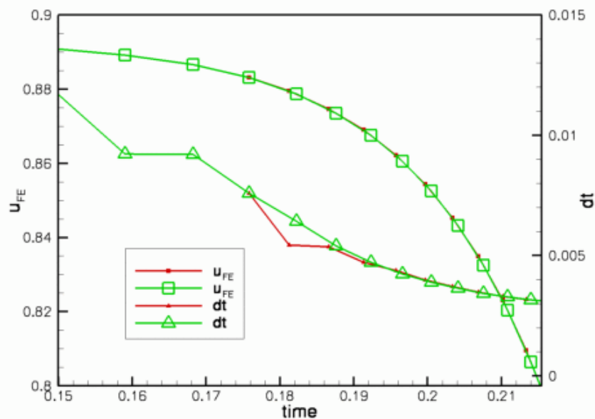
Figure 1.3 Time-trace of the solution and the timestep chosen by the adaptive timestepper in the original (green) and restarted (red) simulation.
